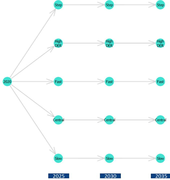
Figure 4.3 2-stage scenario tree problem.
